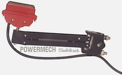
1 Code: DSL-CC-125-STK 125 Amps / 100 Amps Current collector with cable (Model: MACC 125)
